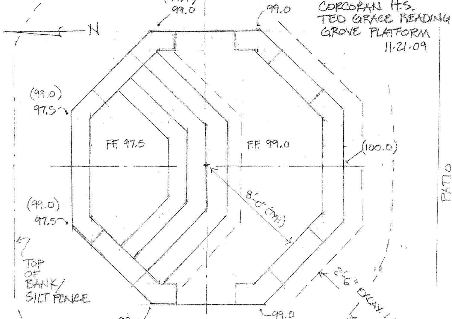
PLAN \frac{1}{4}'' = 1'-0''
